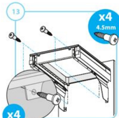
Attach tray with stepped screws
