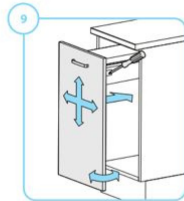
Re-install drawer assembly and adjust door
