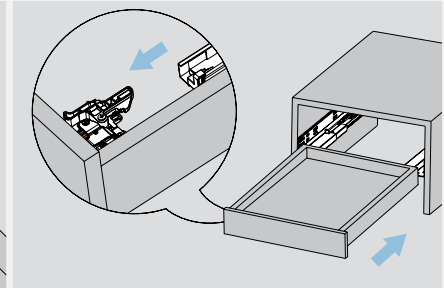
Lay the drawer bottom onto the slide then push the drawer into the cabinet
