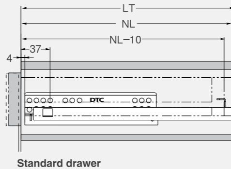
Standard drawer
