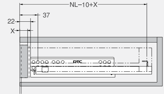
Inner drawer
